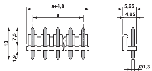
Dimensional drawing
