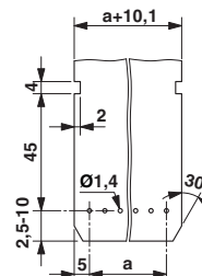
Drilling diagram
