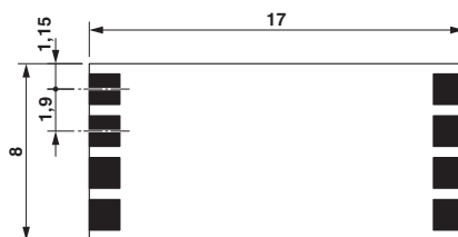
Dimensional drawing
