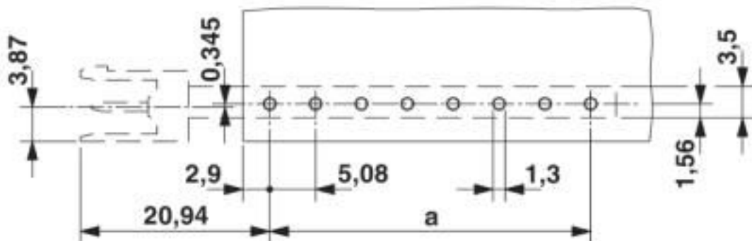
Drilling diagram
