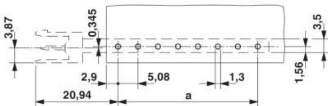
Drilling diagram
