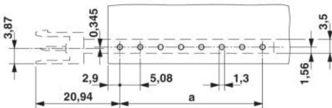
Drilling diagram
