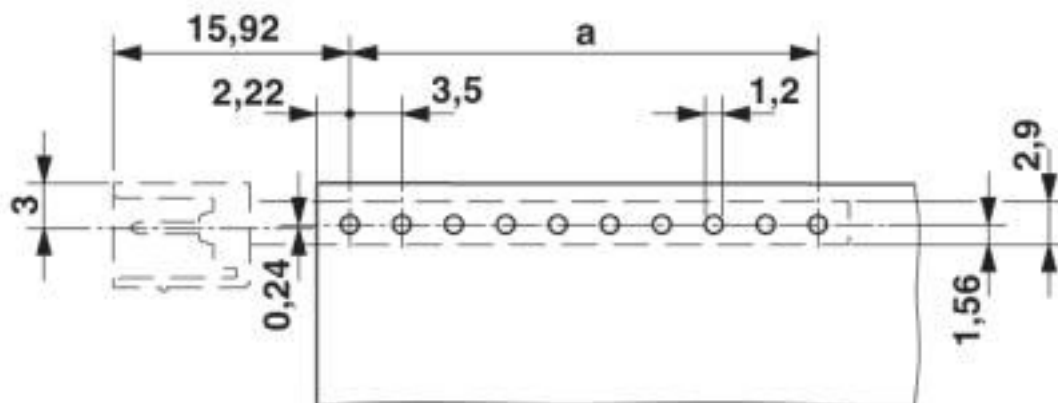
Drilling diagram
