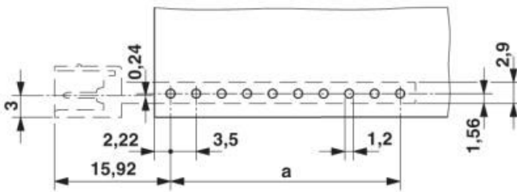
Drilling diagram
