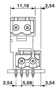
Dimensional drawing
