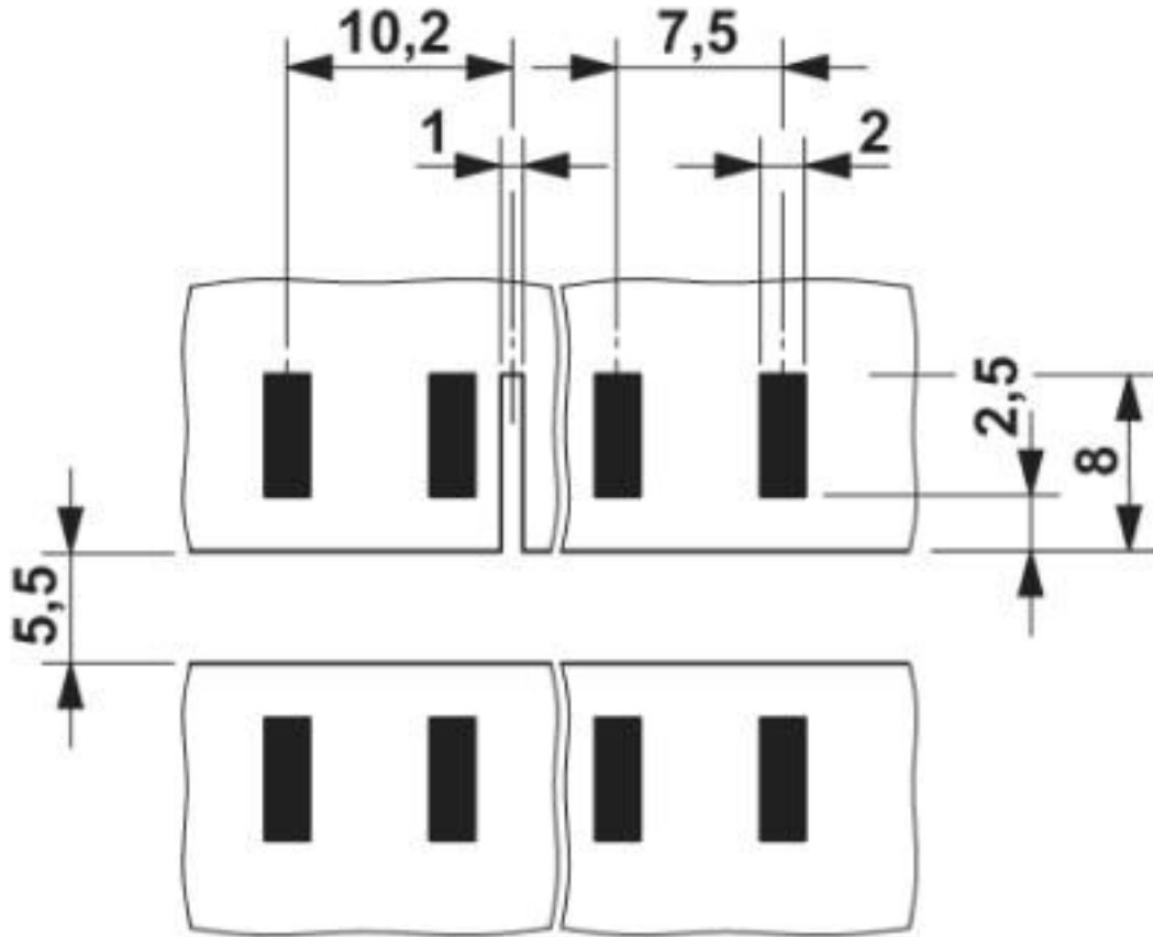
Drilling diagram
