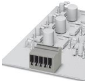
ST-COMBI receptacle, plug-in direction horizontal to the PCB, pitch: 5.2 mm, no. of positions: 9
