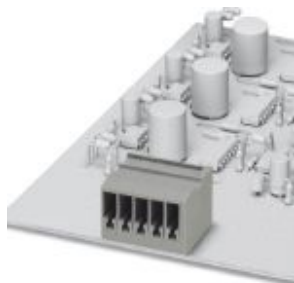
ST-COMBI receptacle, plug-in direction horizontal to the PCB, pitch: 5.2 mm, no. of positions: 11
