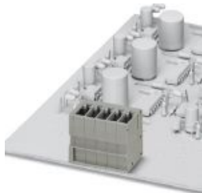
ST-COMBI receptacle, plug-in direction vertical to the PCB, pitch: 5.2 mm, no. of positions: 11
