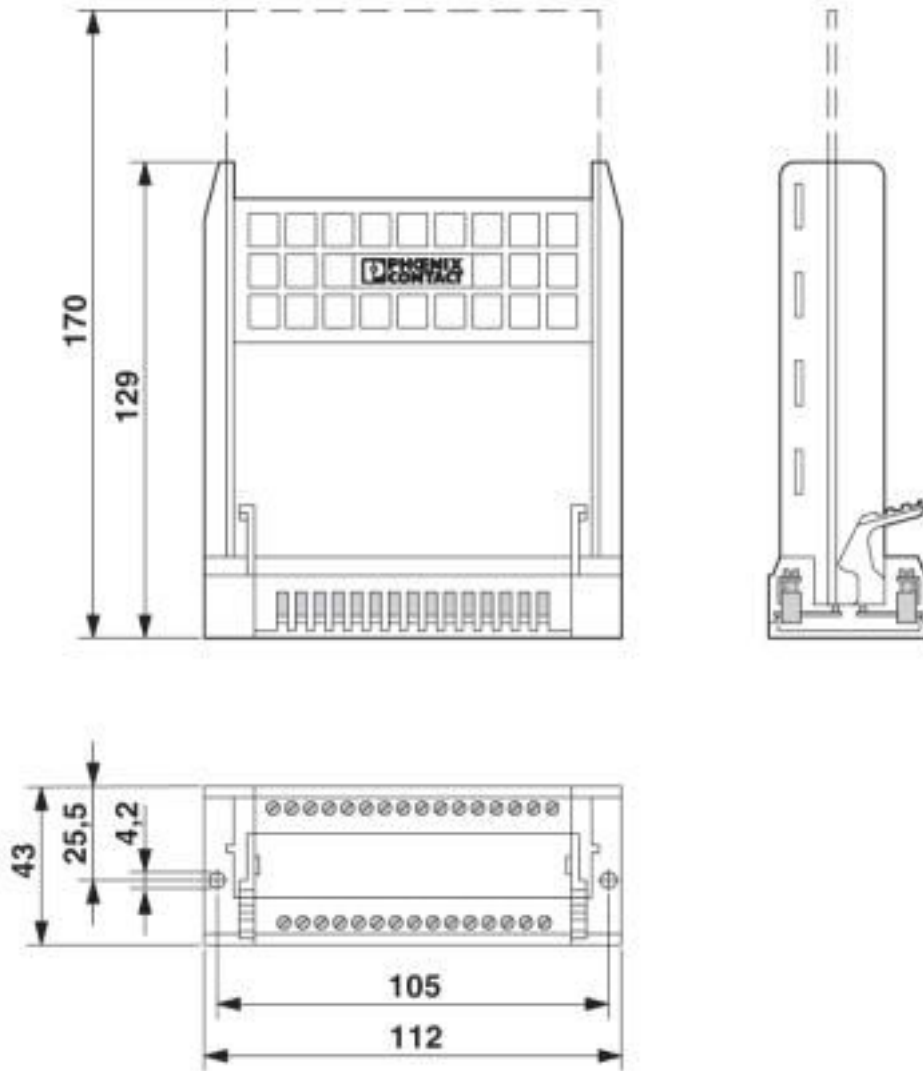
Dimensional drawing
