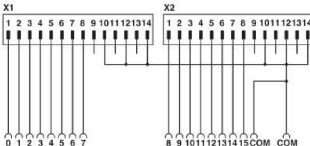
Connection scheme FLKM 14-PA-SLC500/IN
