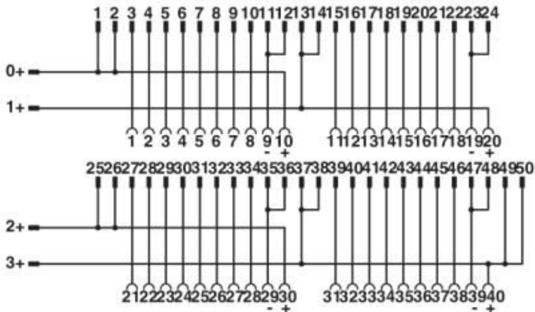
Connection scheme FLKM 50-PA-MODI-TSX/Q
