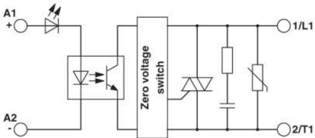
Block diagram
