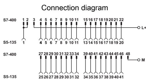
Connection scheme: FLKM S135/S400/SO120
