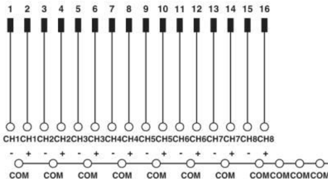
FLKM 16/AI/DV connection scheme
