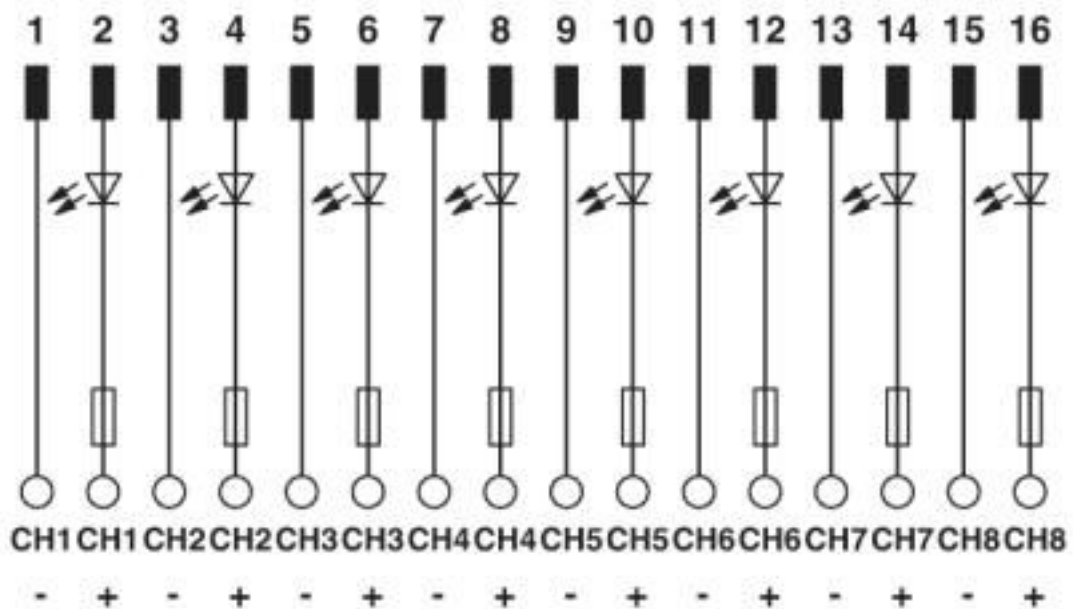
FLKM 16/DI/SI/LA/DV connection scheme
