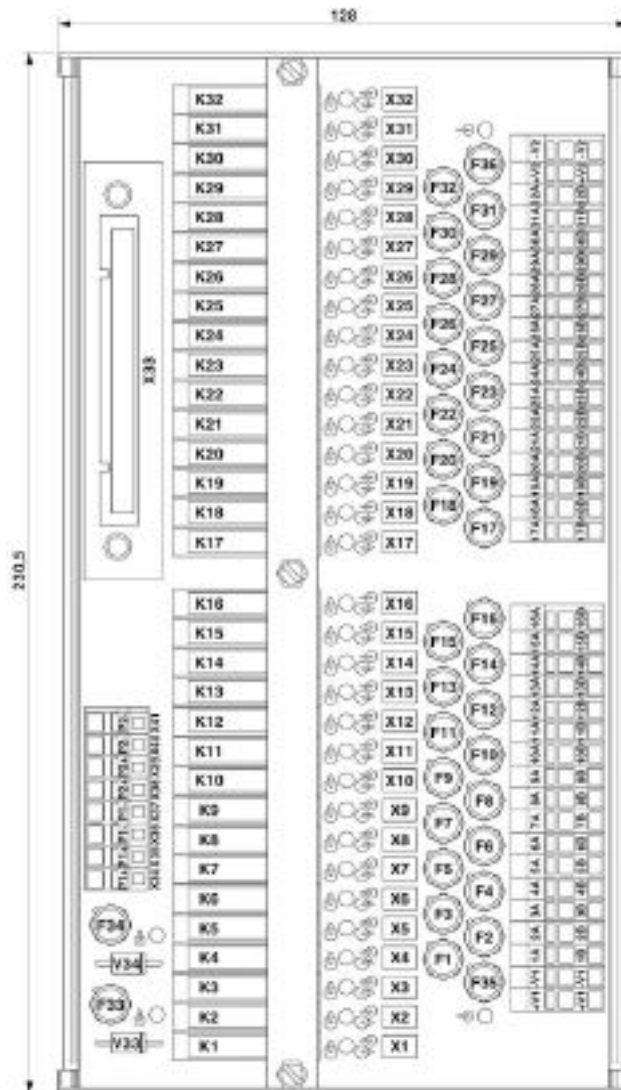
Dimensional drawing
