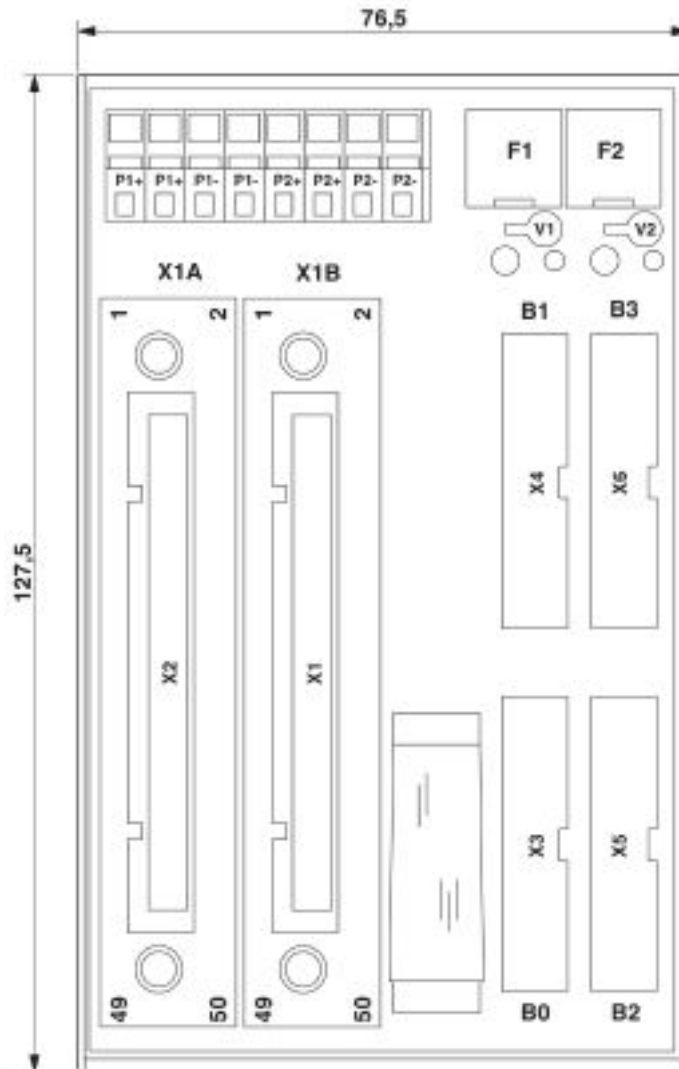
Dimensional drawing
