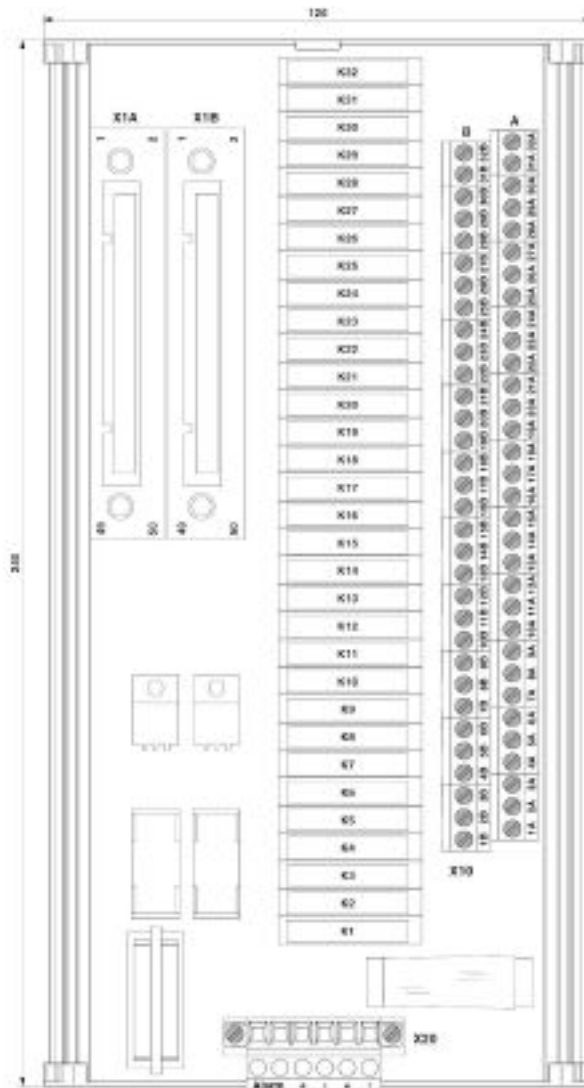
Dimensional drawing
