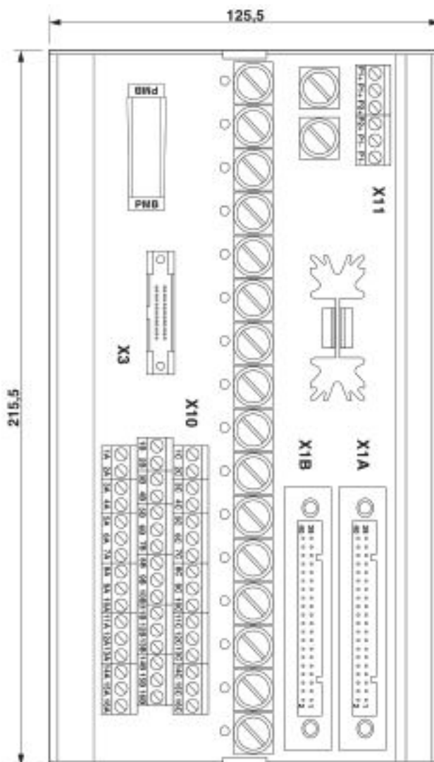
Dimensional drawing
