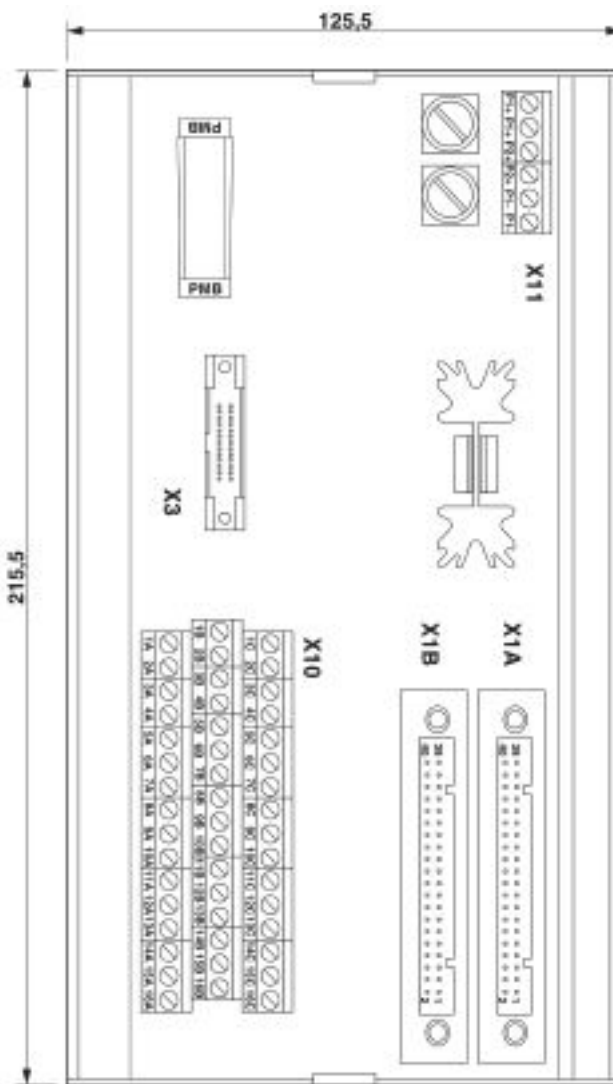
Dimensional drawing
