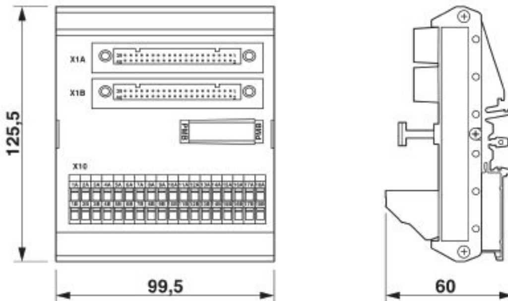
Dimensional drawing
