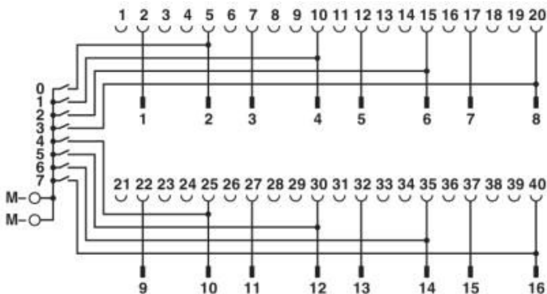
Connection scheme FLKM 16-PA-331-1KF//MINI-MCR
