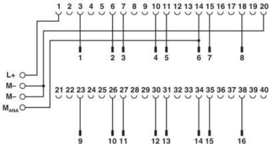
Connection scheme FLKM 16-PA-332-5HF/I/MINI-MCR
