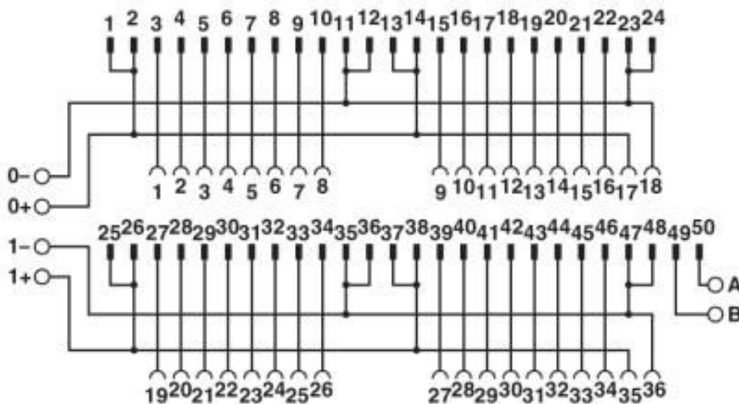
Connection scheme for FLKM 50-PA-GE/TKFC/RXI
