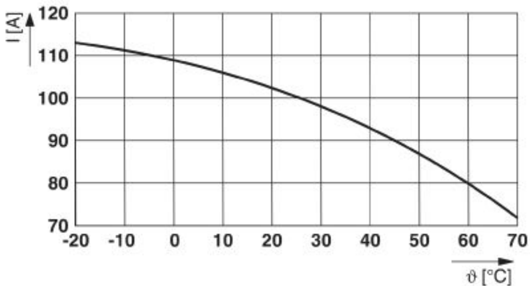
Derating curve: 100 mA fuse
