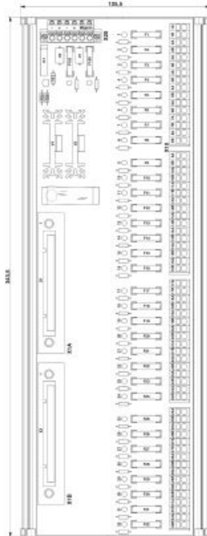
Dimensional drawing
