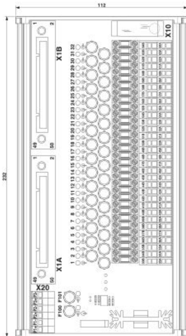
Dimensional drawing
