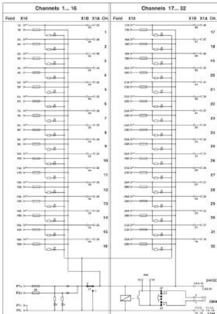
Circuit diagram
