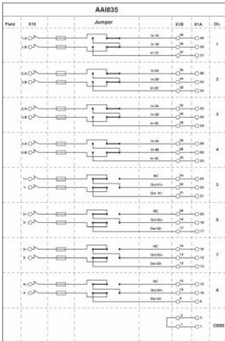
Circuit diagram
