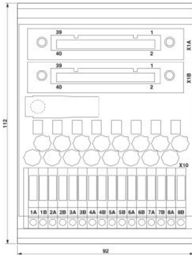
Dimensional drawing
