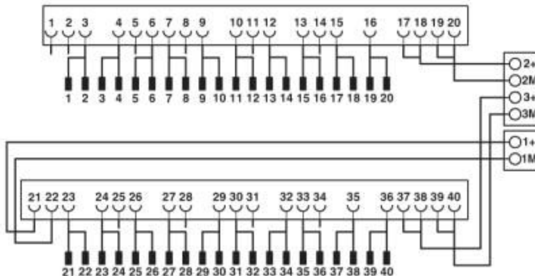
Connection scheme FLKM 50-PA/DO326/S7-300
