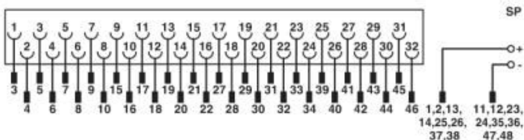
Circuit diagram
