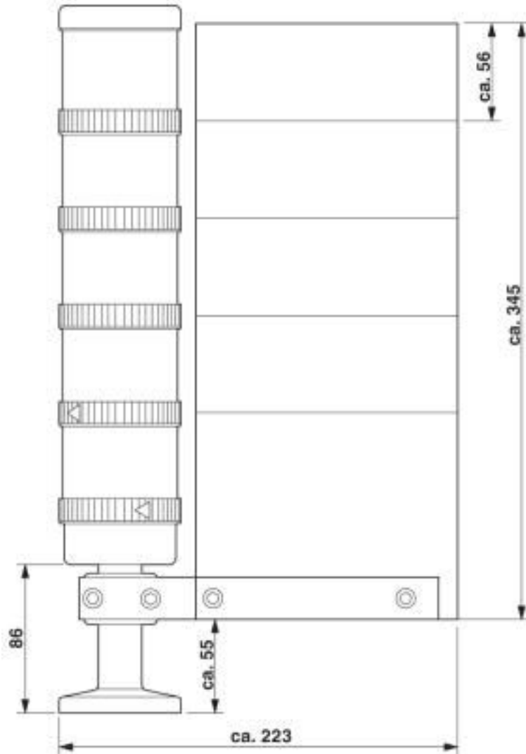
Dimensional drawing
