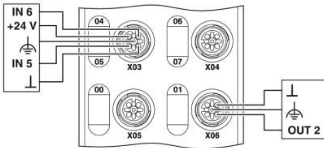
Connection diagram
