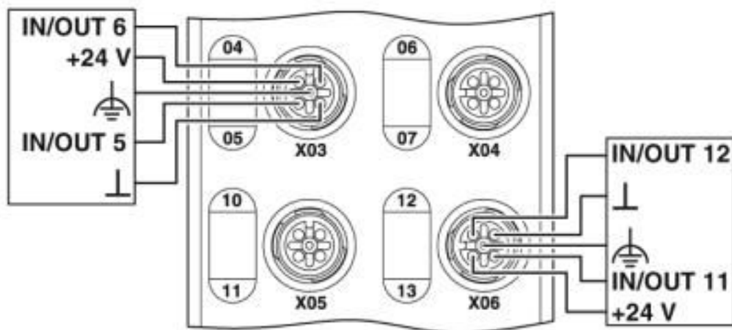
Connection diagram
