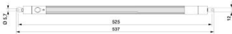
Dimensional drawing
