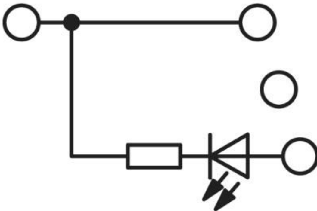
Circuit diagram
