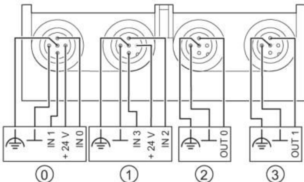
Connection diagram
