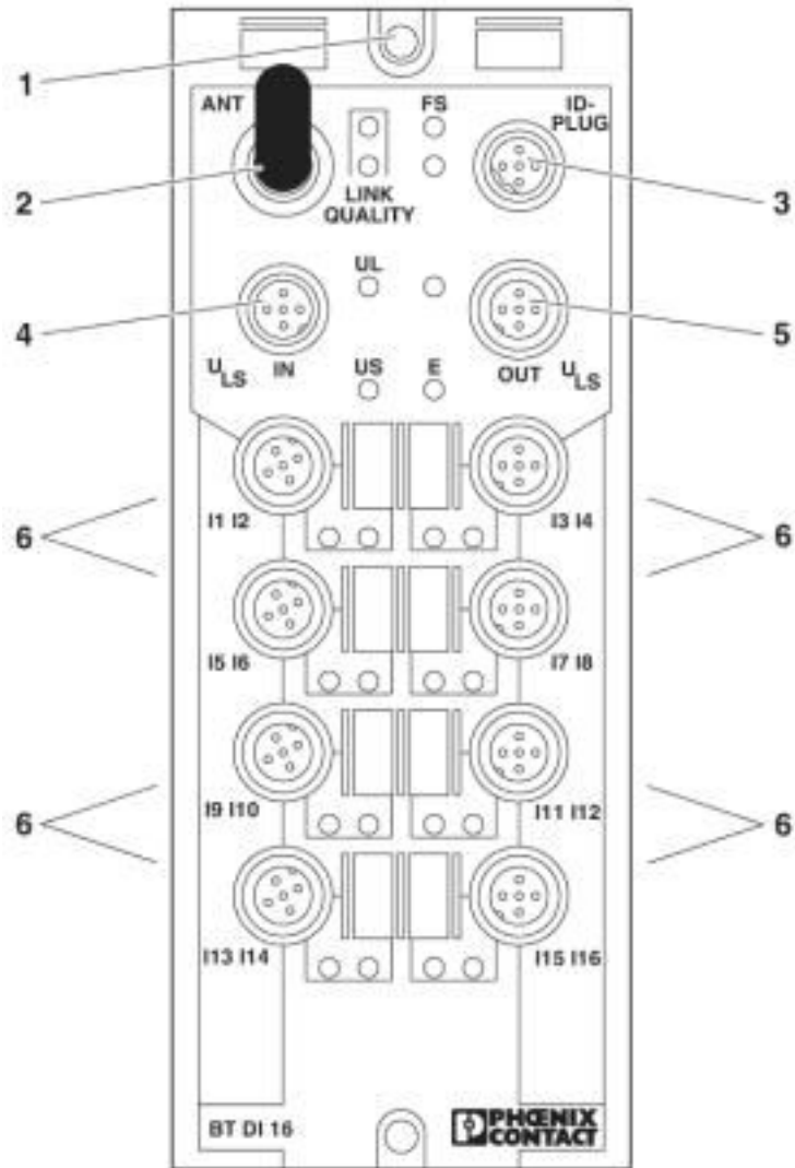
Product drawing
