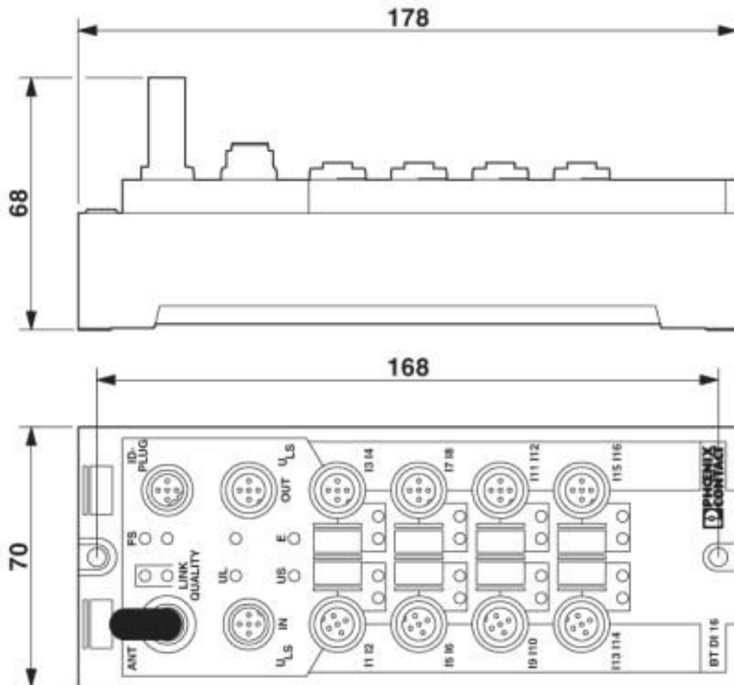
Dimensional drawing
