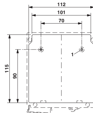
1 = Diameter 3.2 mm for M3
