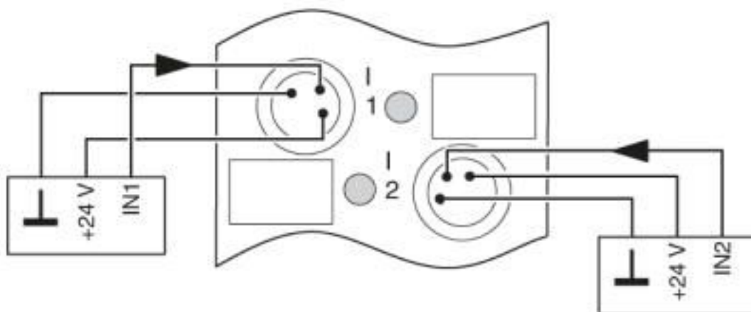
Connection diagram
