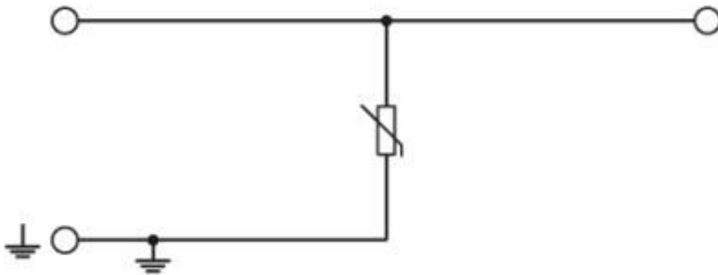
Circuit diagram
