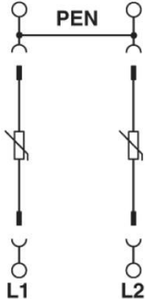
Circuit diagram
