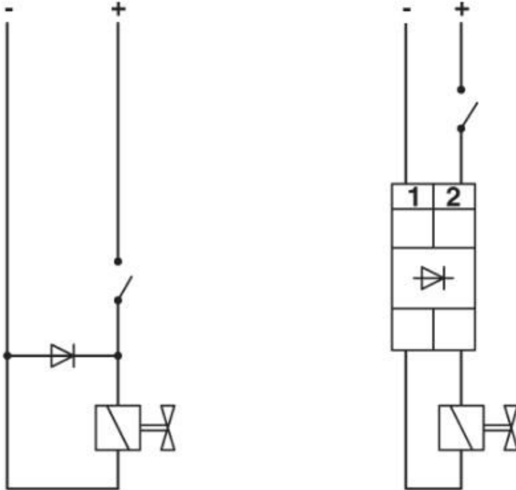
Circuit diagram
