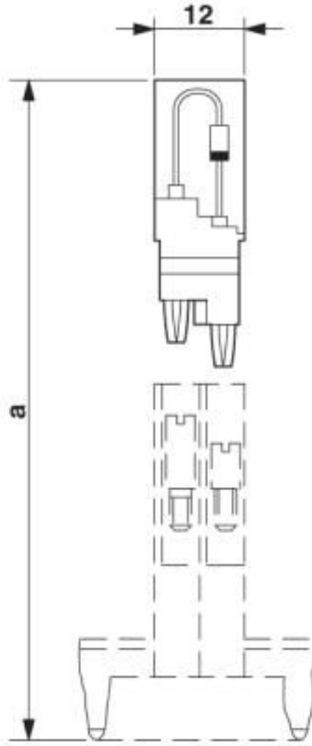
Dimensional drawing
