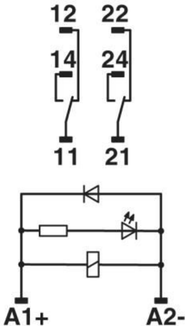
Circuit diagram
