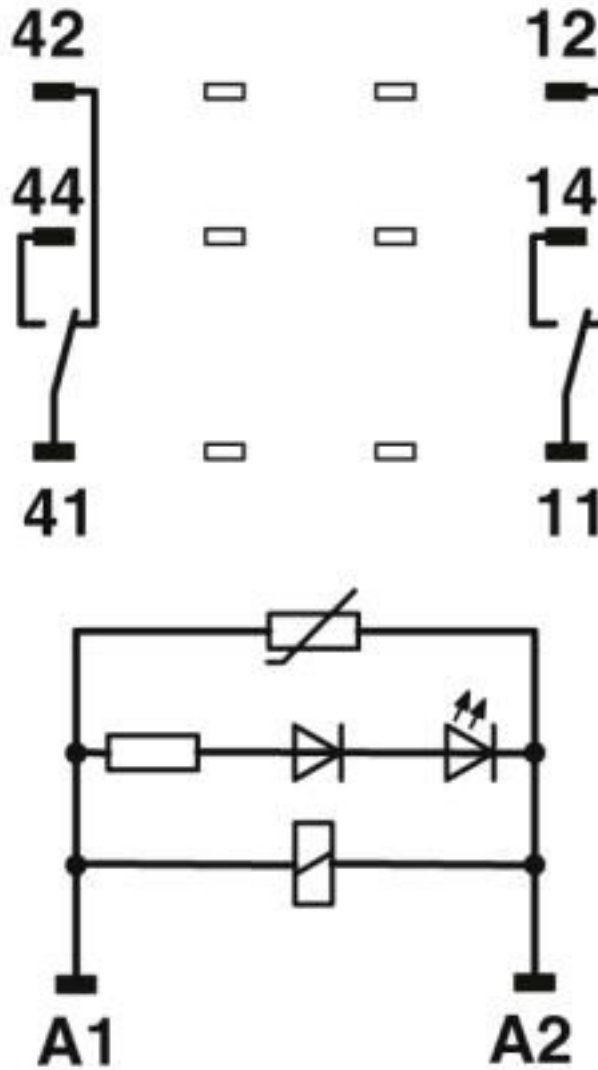
Circuit diagram
